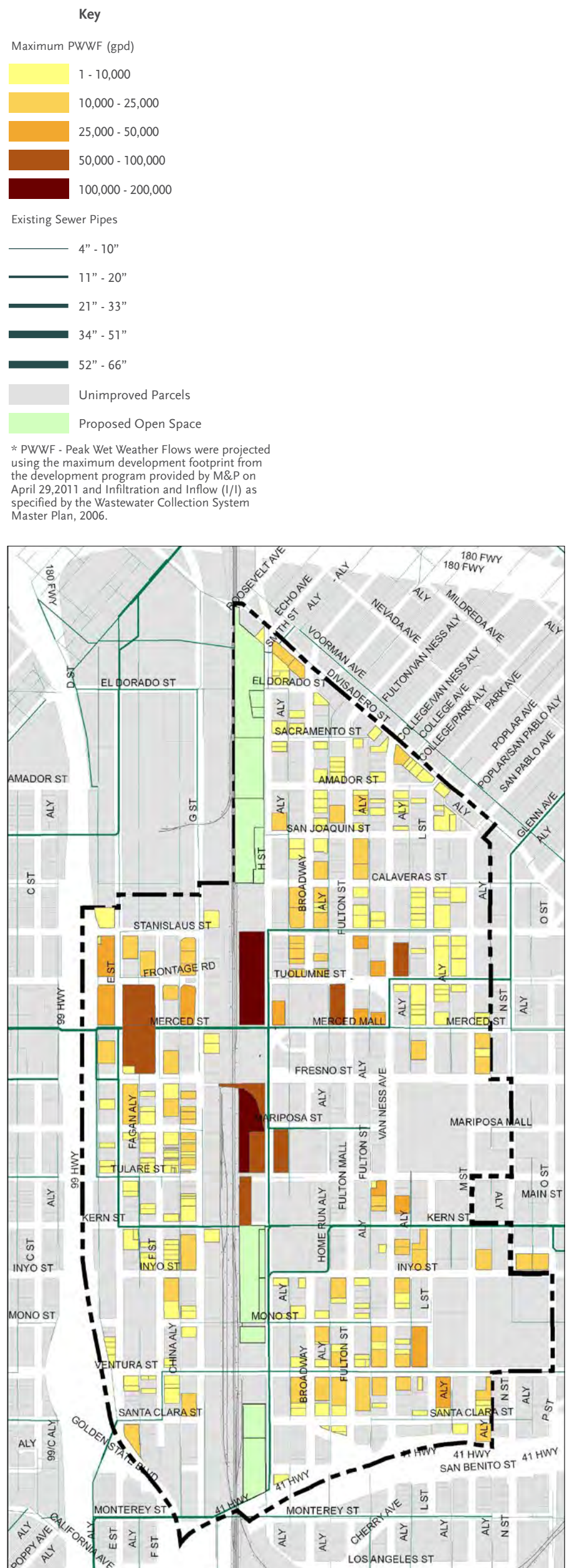
Figure 11.9C - Existing Sewer Infrastructure and Projected Demand
