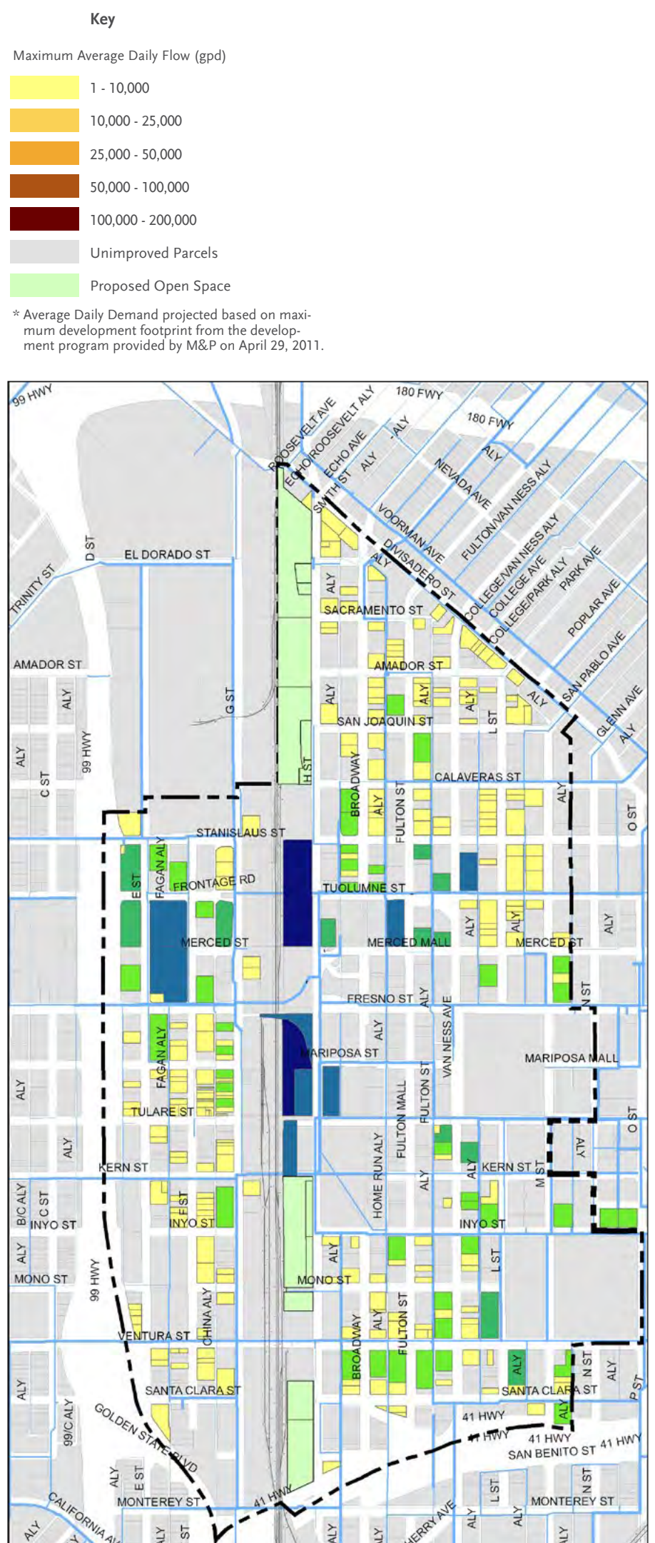
Figure 11.9A - Existing Water Infrastructure and Projected Demand
