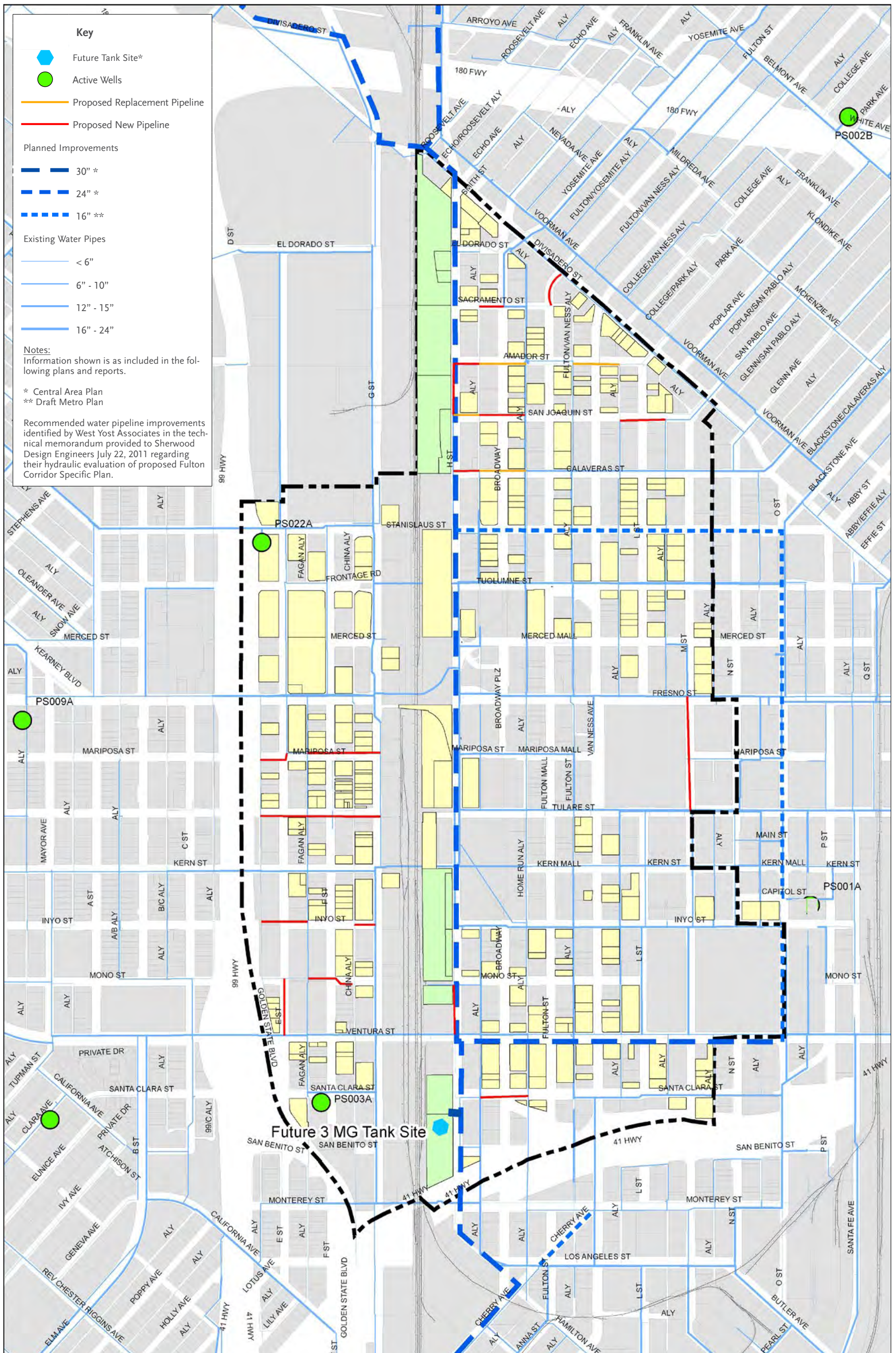
Figure 11.9B - Water Infrastructure & Required Water Infrastructure Improvements
